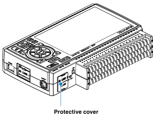
Protective cover
